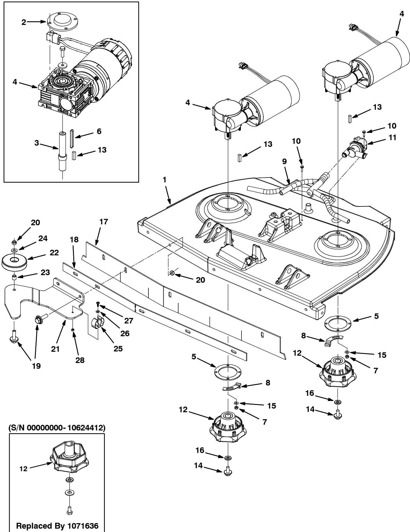
Fig. 17 - Disk Scrub Head Drive Motor Group, 800 mm (32 in)
