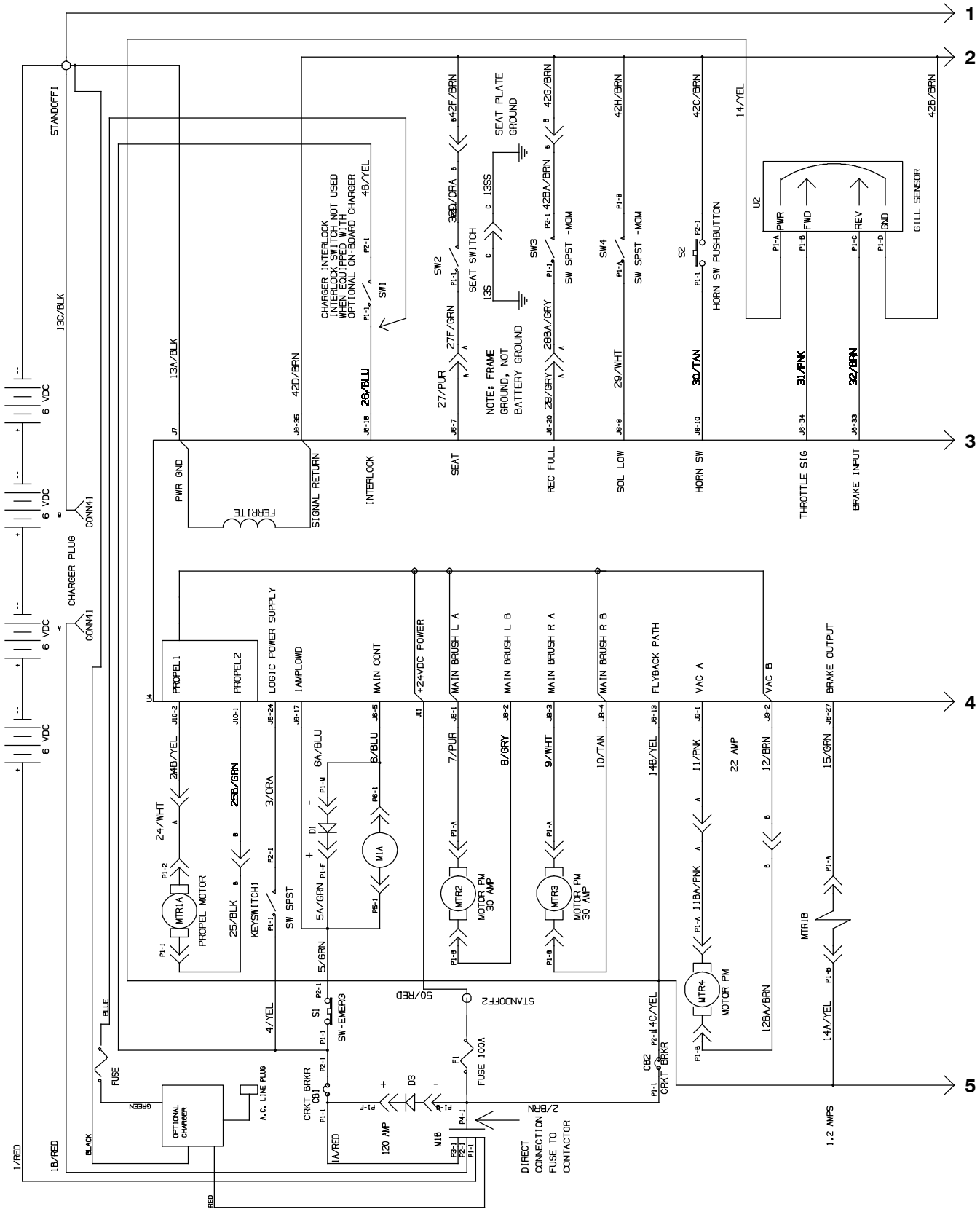
Fig. 40 - Electrical Schematic, Standard & FaST Model (S/N 00000000- 10426042)
