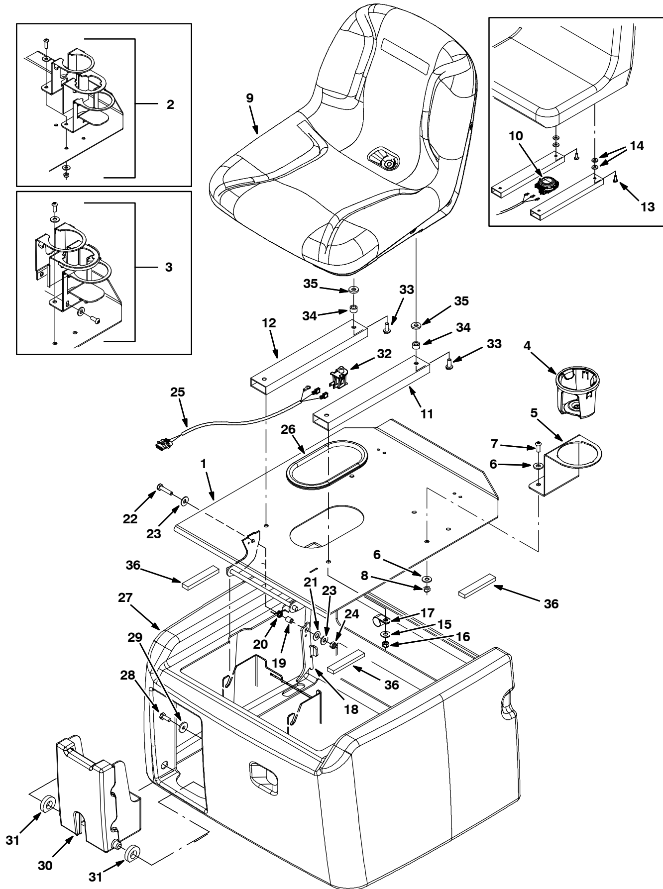
Fig. 7 - Seat Group
