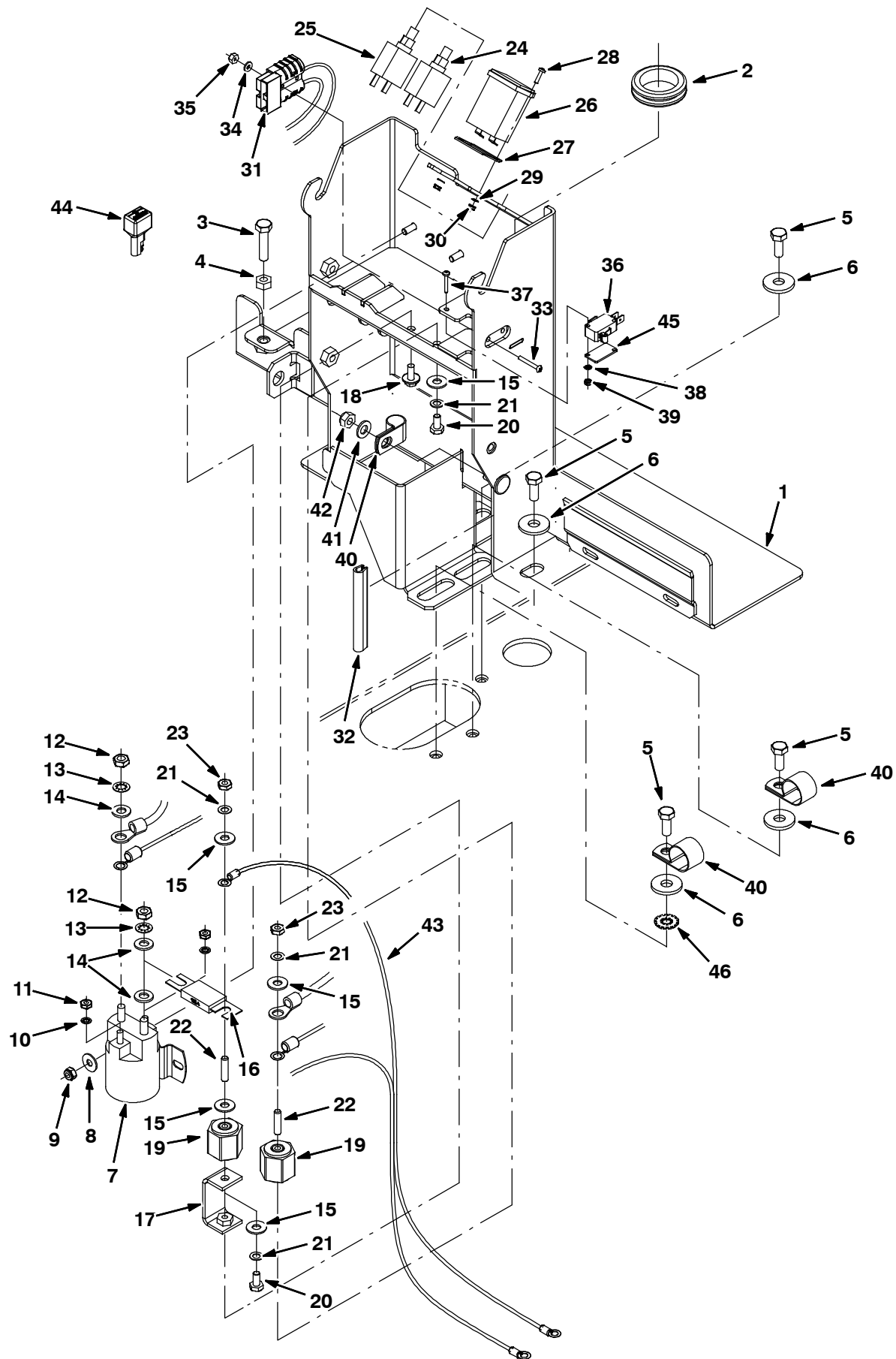
Fig. 38 - Electrical Group
