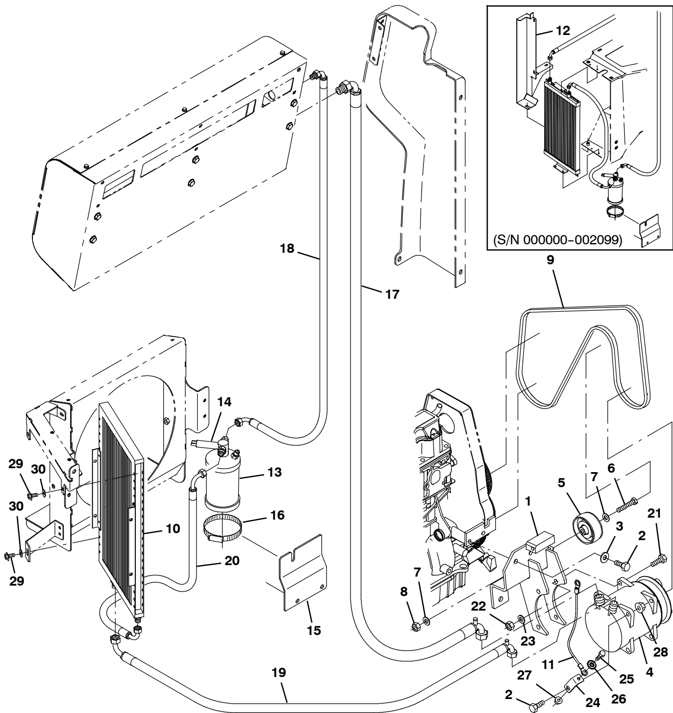
Fig. 14 - Cab Air Conditioner Group (000000-005699)
