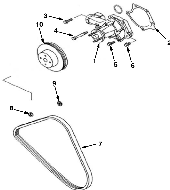
Fig. 9 - Water Pump Group
