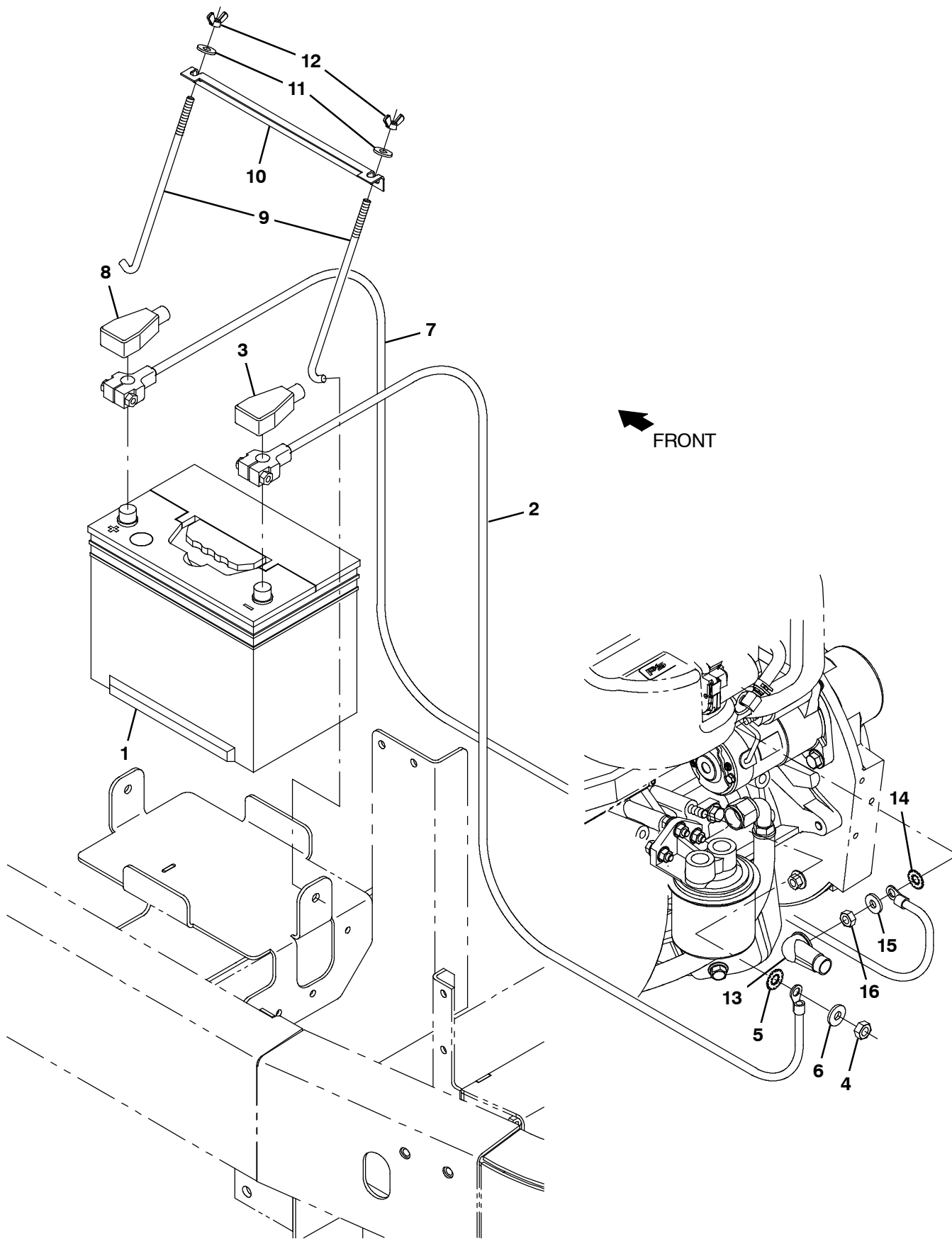
Fig. 34 - Engine Battery Group (005700- )
