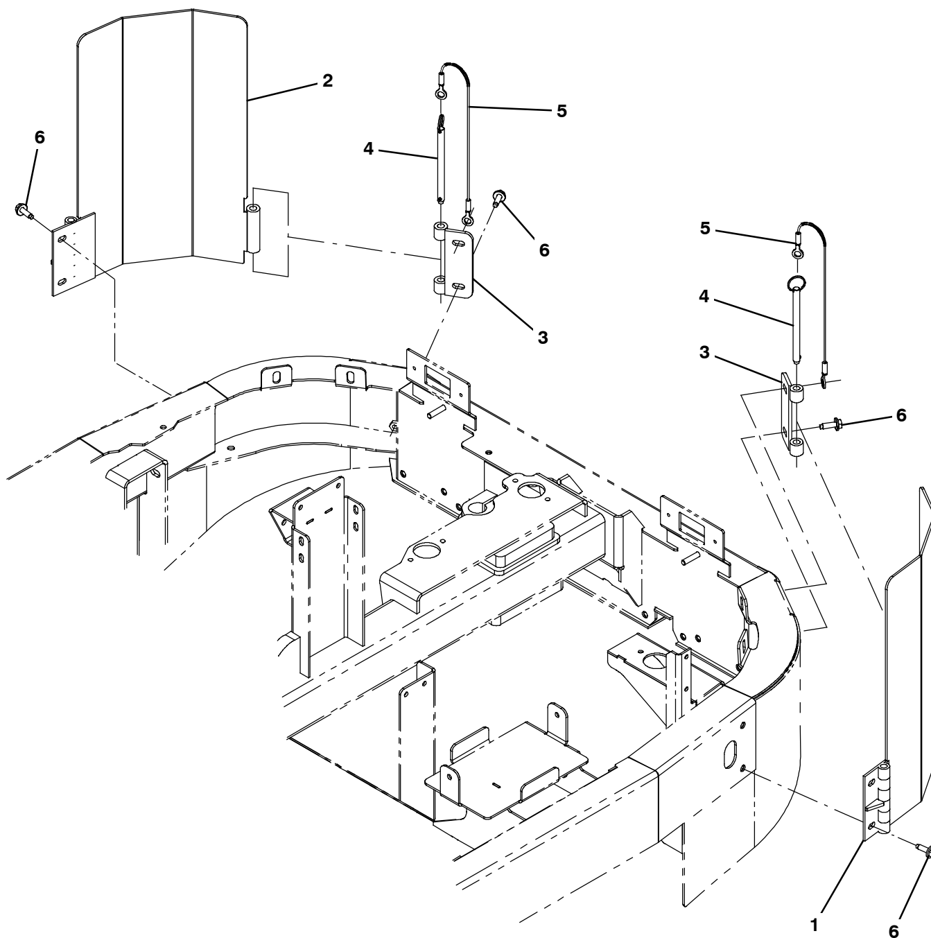
Fig. 19 - Corner Bumper Kit (000000-002099)
