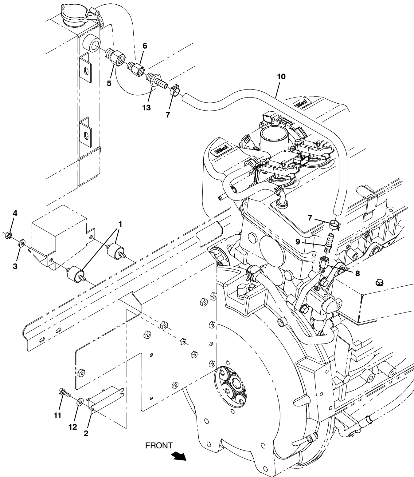
Fig. 23 - Engine EFI Group, Gas (005700- )
