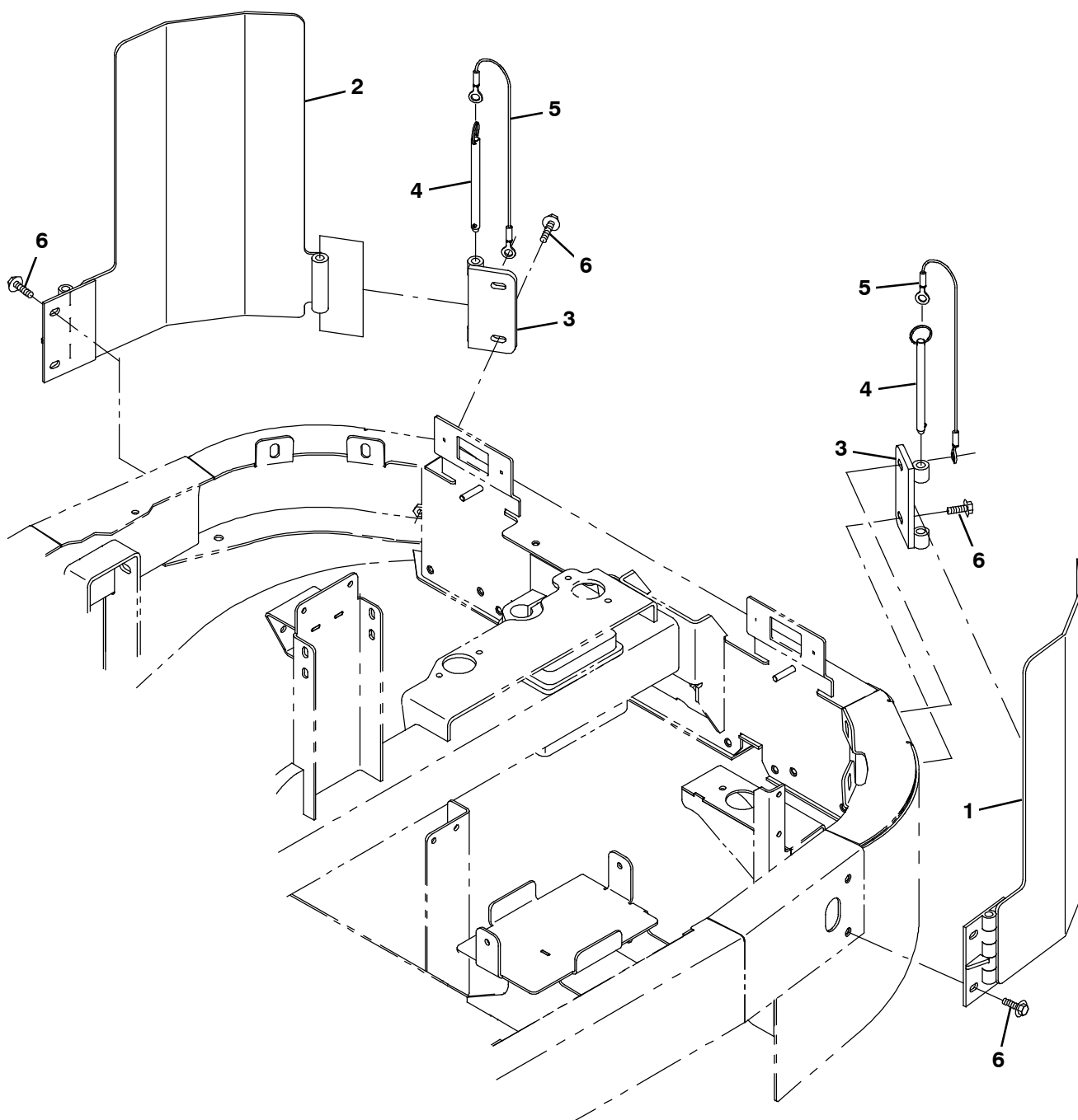
Fig. 20 - Corner Bumper Kit (002100- )
