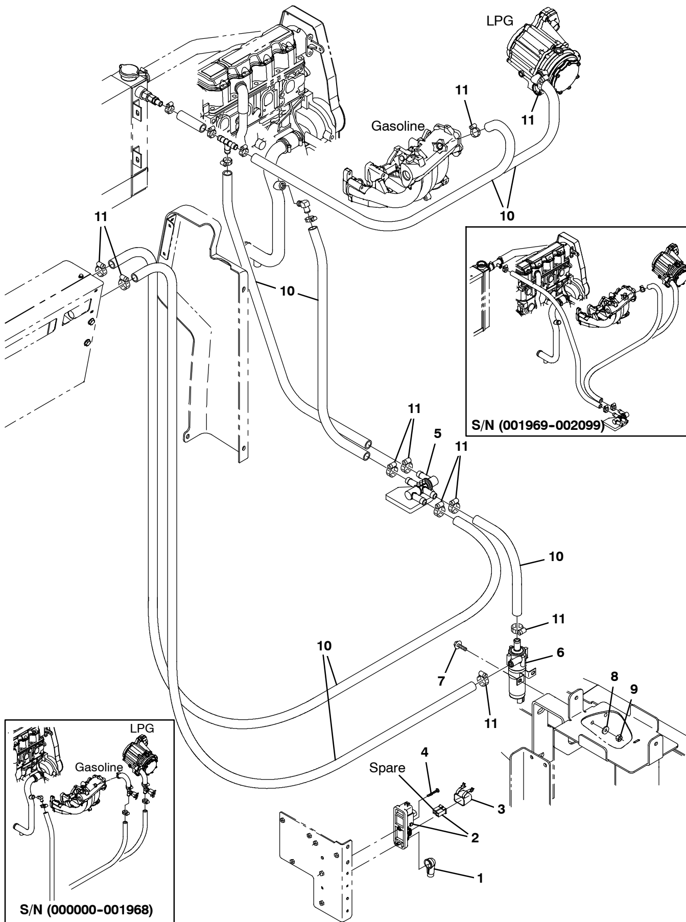
Fig. 13 - Cab Heater Group
