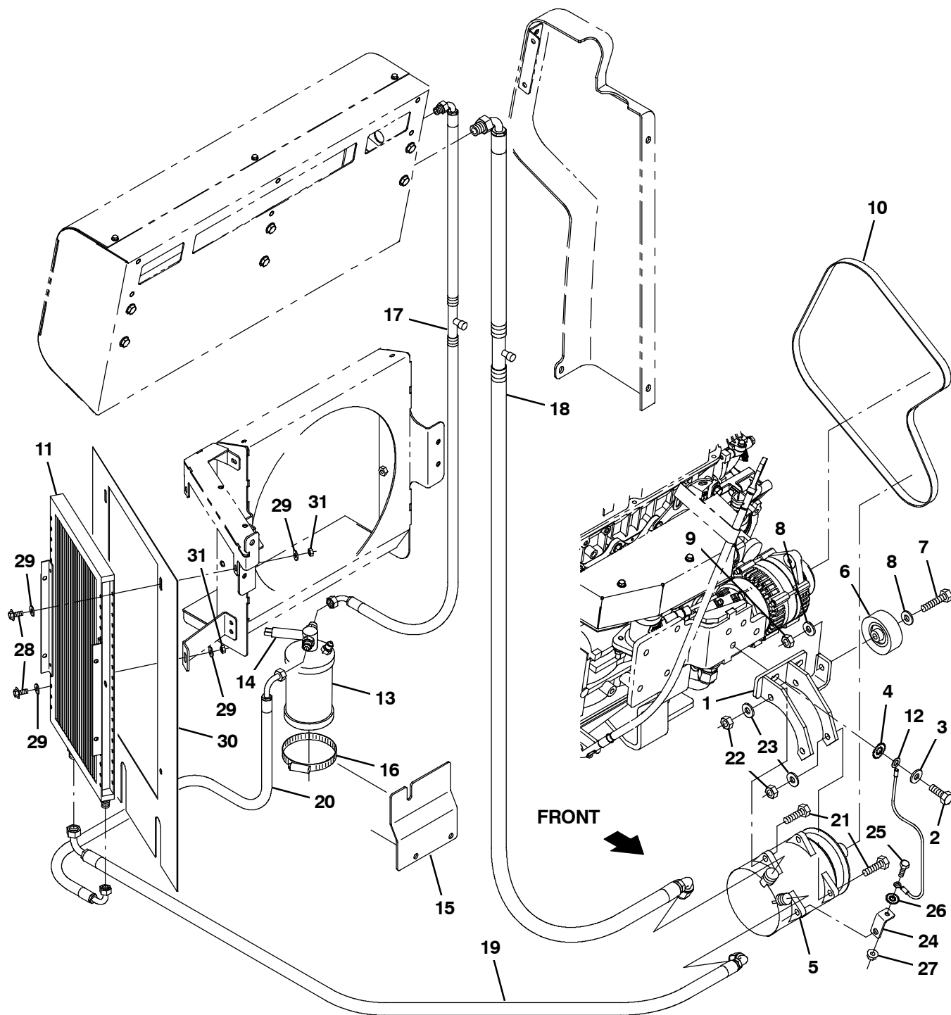
Fig. 15 - Cab Air Conditioner Group (005700- )
