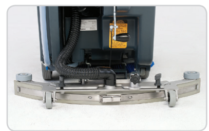
Tool-less squeegee blades can be rotated for use on both sides to save replacement costs.
