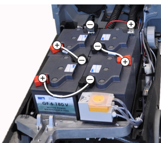
Installation sketch for 4 batteries
