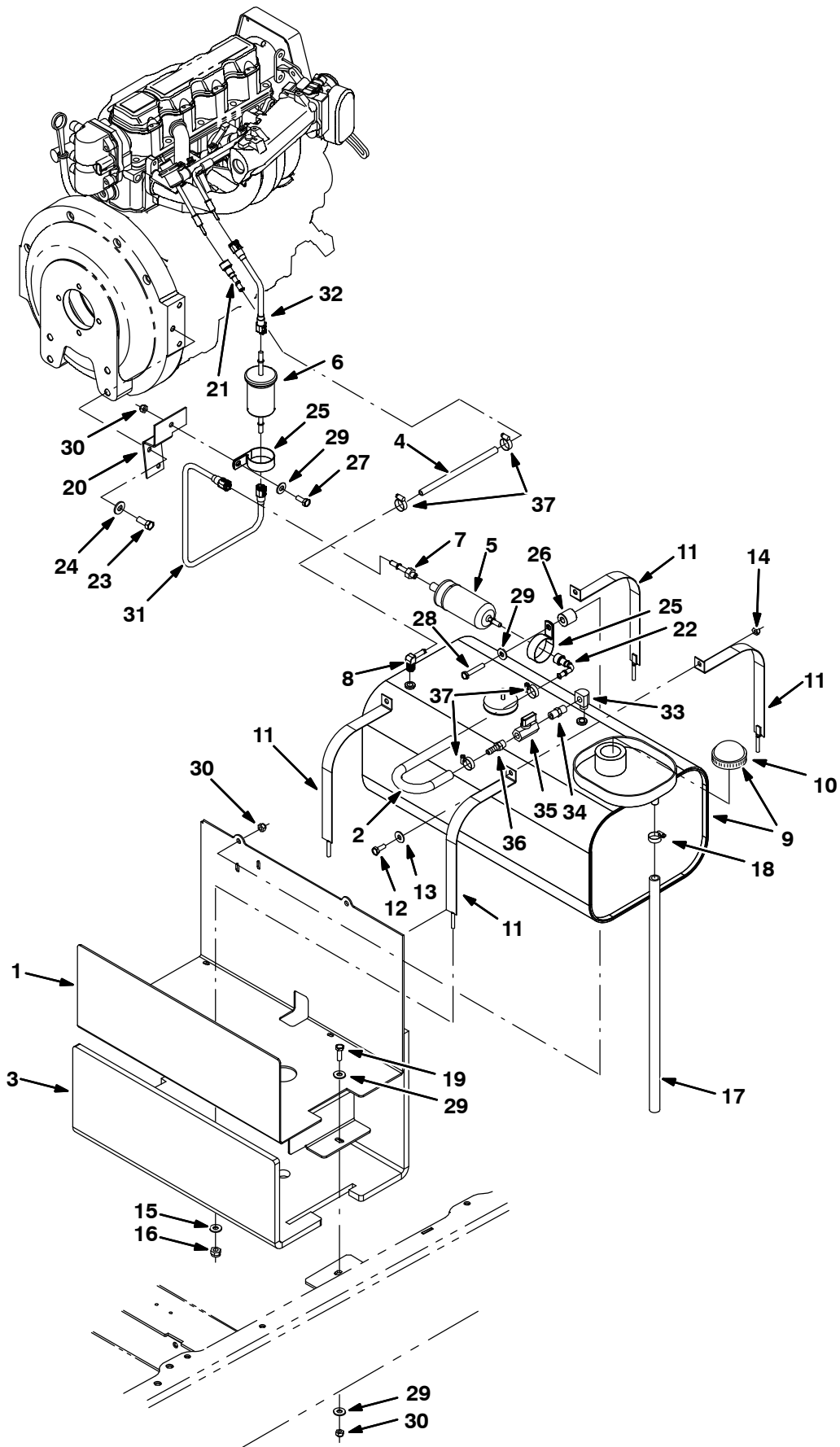
Fig. 39 – Engine Fuel Tank Group, Gasoline (000000–001999)
