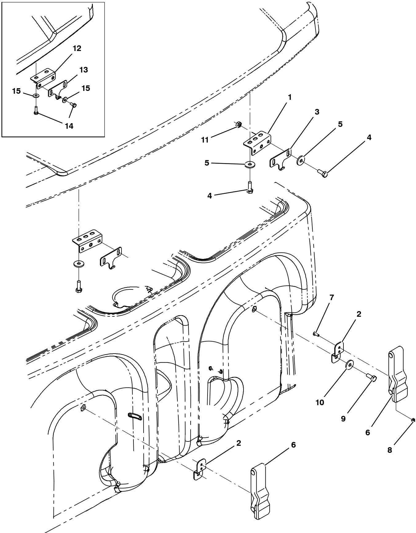
Fig. 34 – Transport Group
