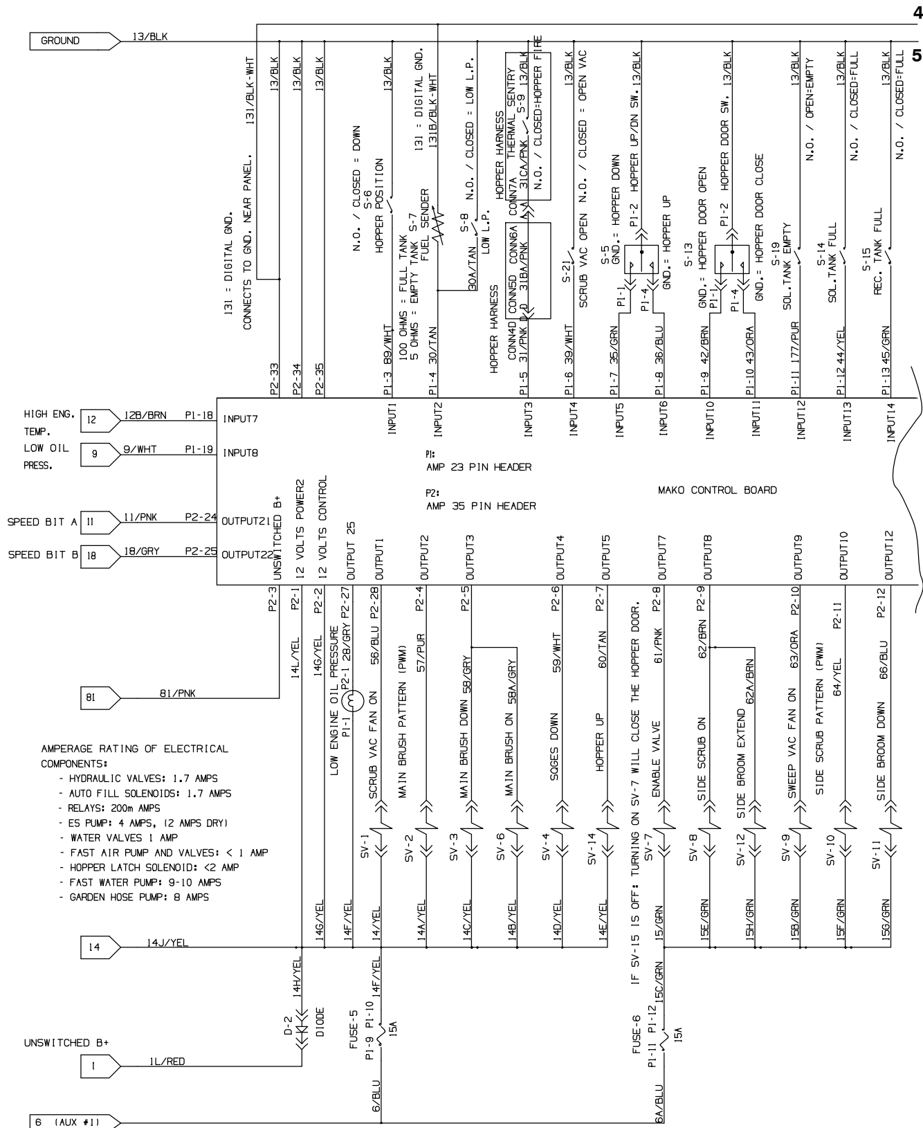
Fig. 86 – GM Electrical Schematic (000000–001999)
