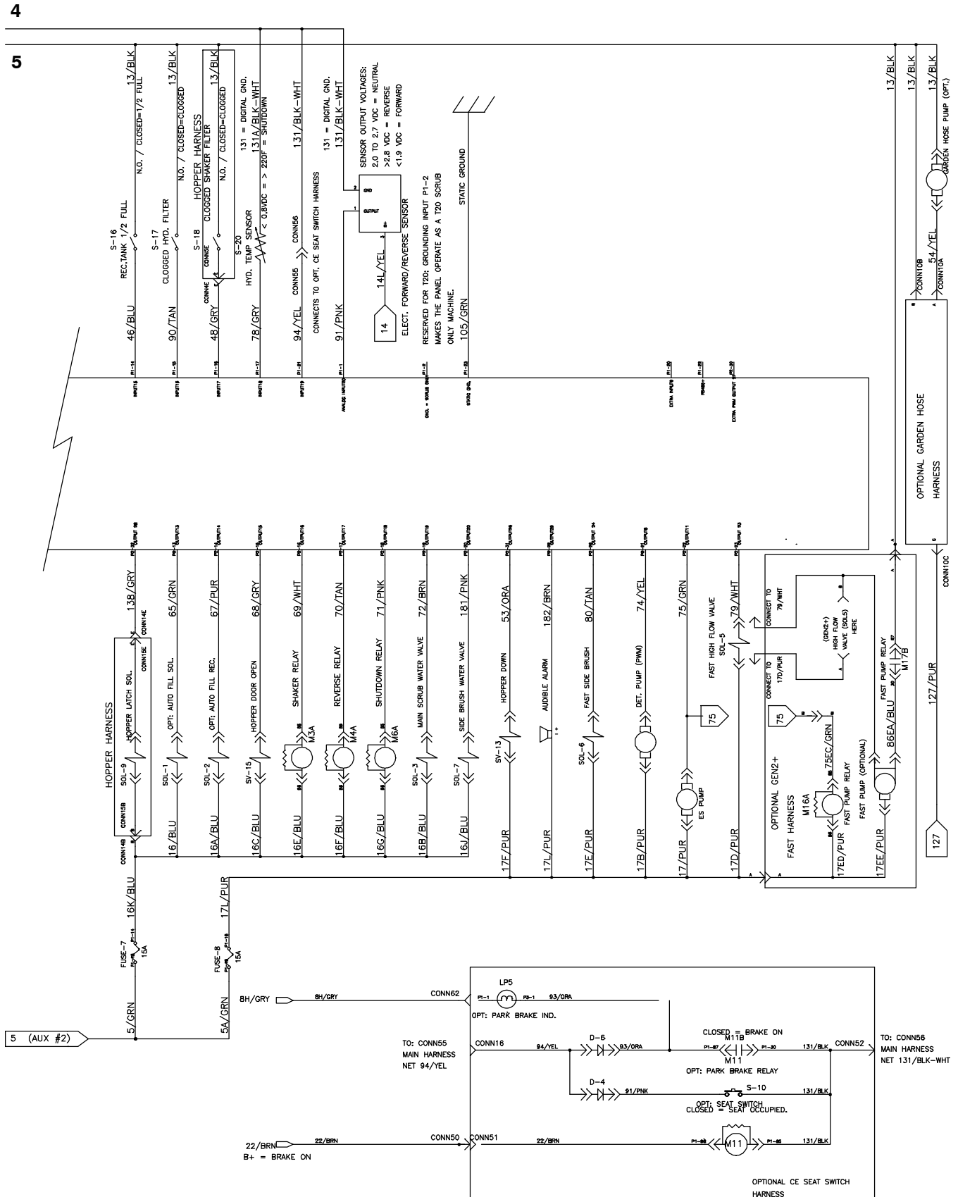
Fig. 88 – GM Electrical Schematic (002533–005999)
