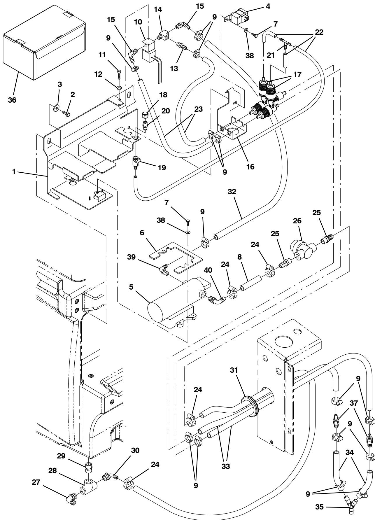
Fig. 14 – FaST Pumps and Detergent Group (002533– )
