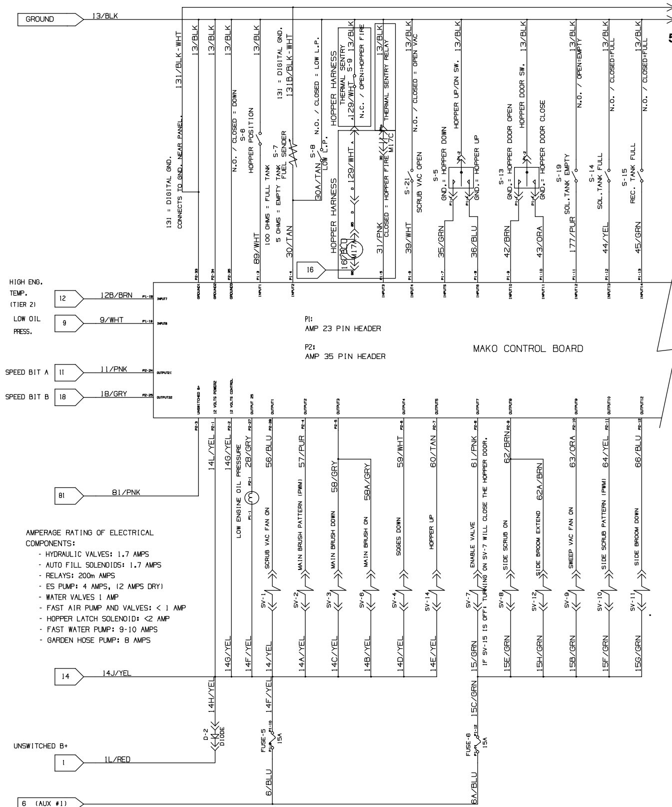
Fig. 89 – GM Electrical Schematic (003479–005999)
