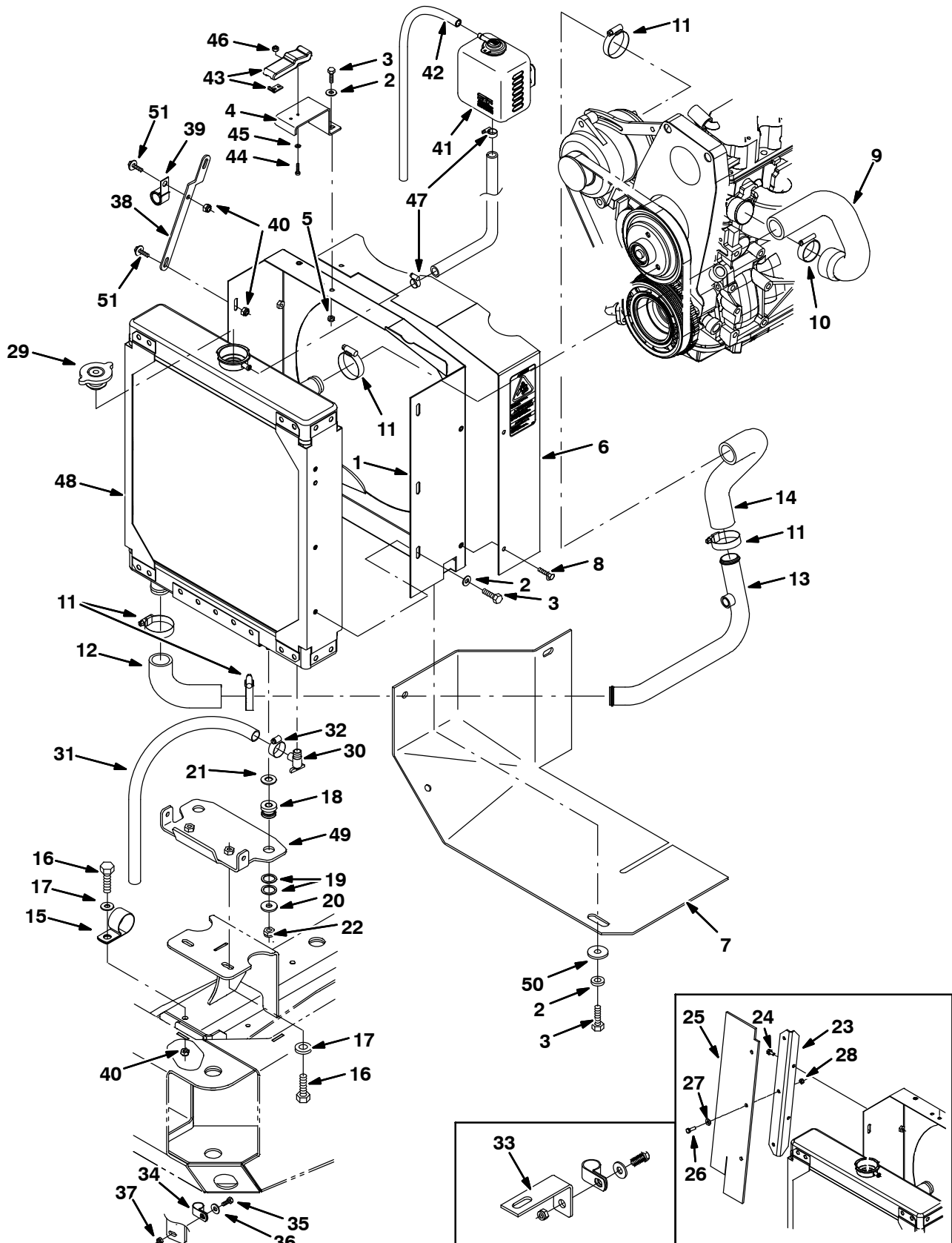
Fig. 26 – GM Engine Radiator Group (000000-003038)
