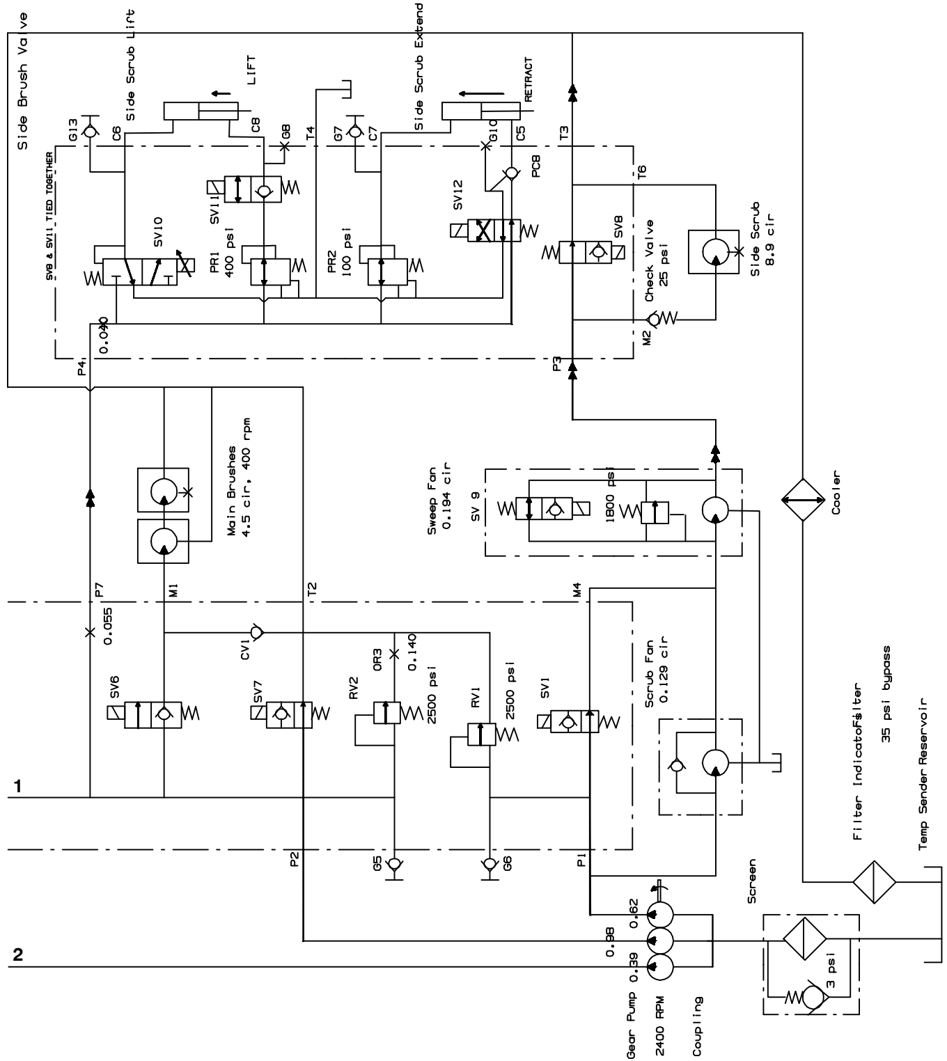
Fig. 75 – Hydraulic Schematic (003298– )
