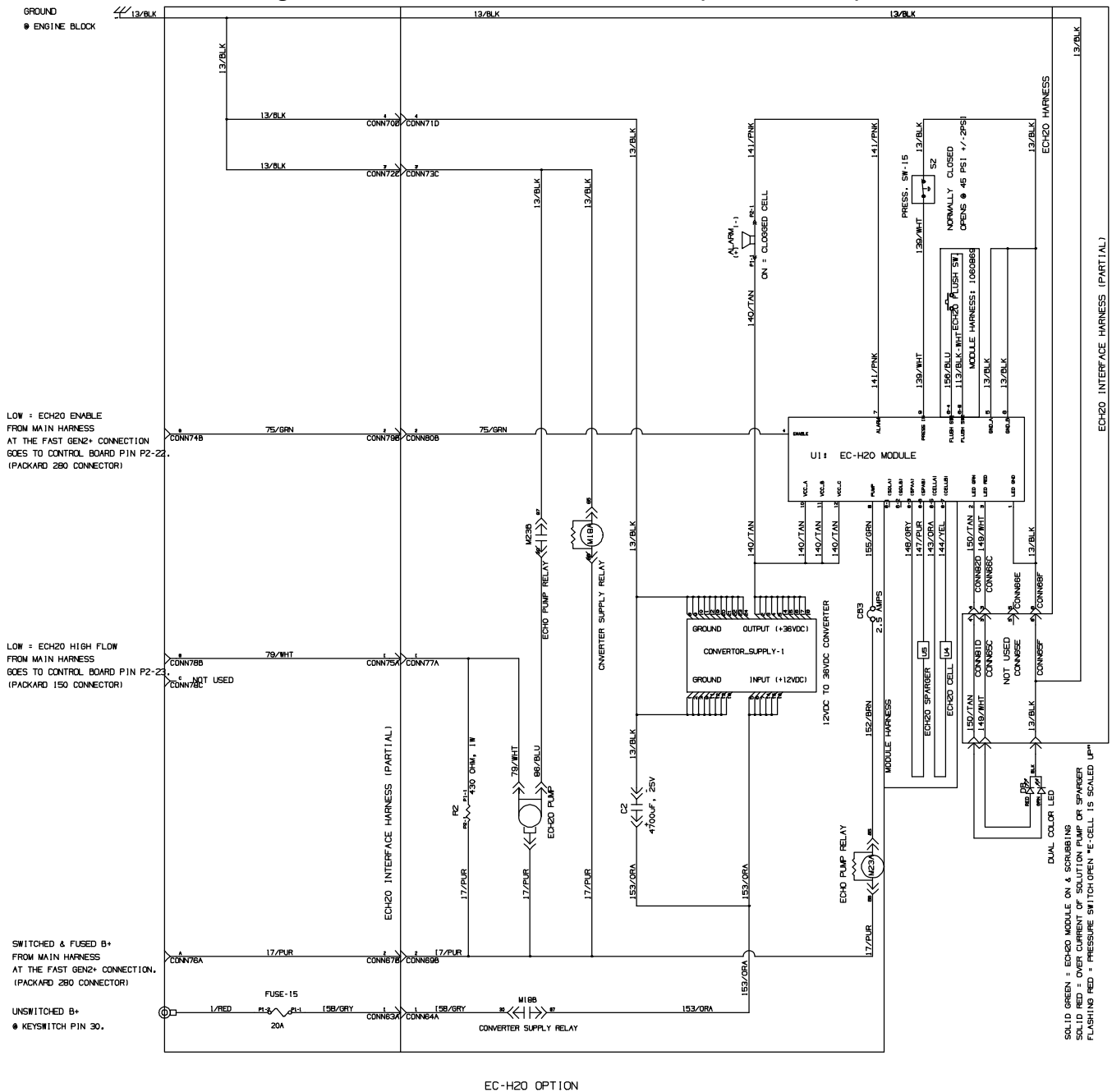
Fig. 95 – Mitsubishi Electrical Schematic (006000– )
