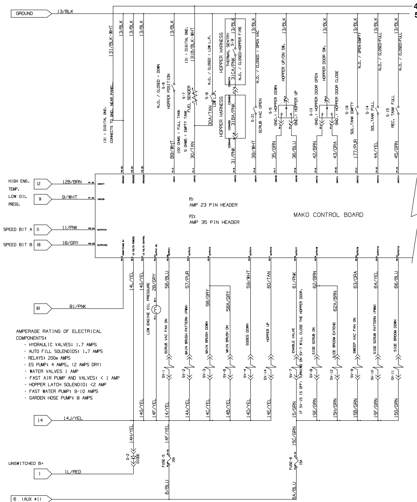
Fig. 87 – GM Electrical Schematic (002000–002532)
