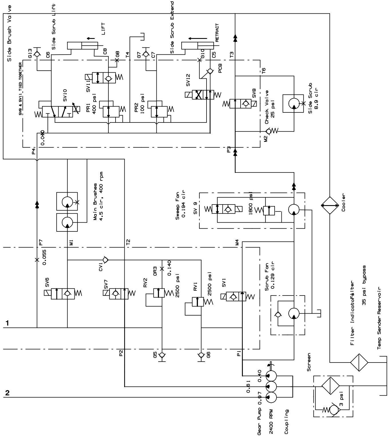
Fig. 74 – Hydraulic Schematic (002700–003297)
