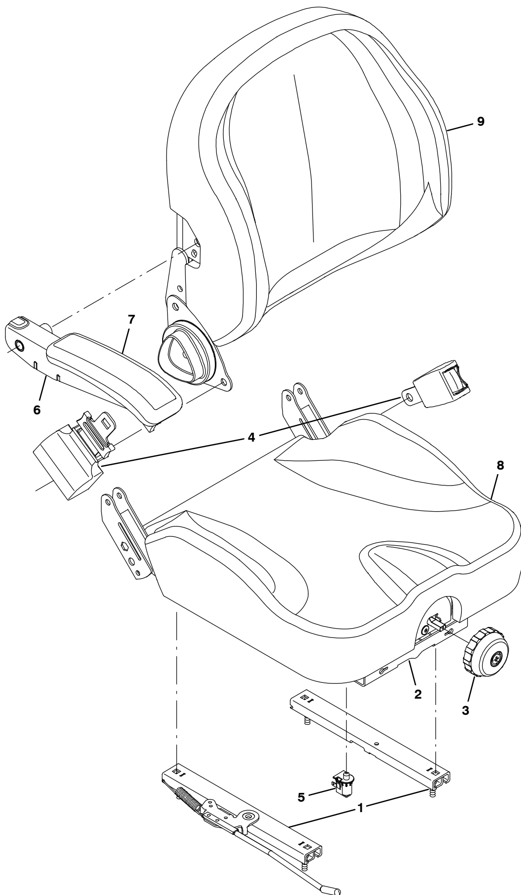
Fig. 18 – Seat Breakdown, 1072456
