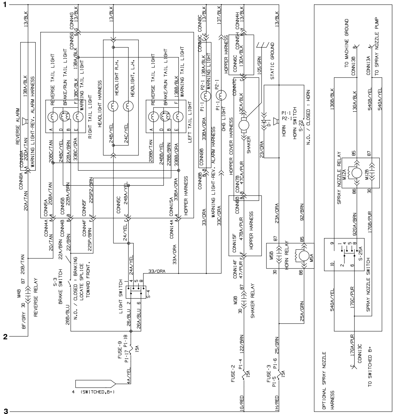
Fig. 86 – GM Electrical Schematic (000000-001999)
