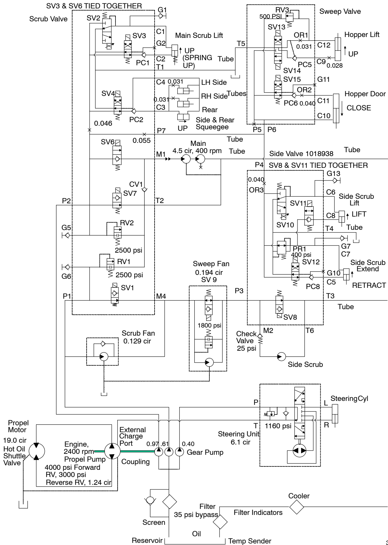
Fig. 73 – Hydraulic Schematic (000000–002699)
